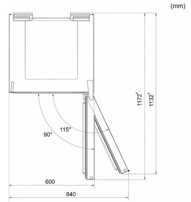
KD26022Sws, KD26022Sedo, KD28032, KF28032D, KFN29032, KFN29042; KFN29032, (schéma) (*note en bas de page)
